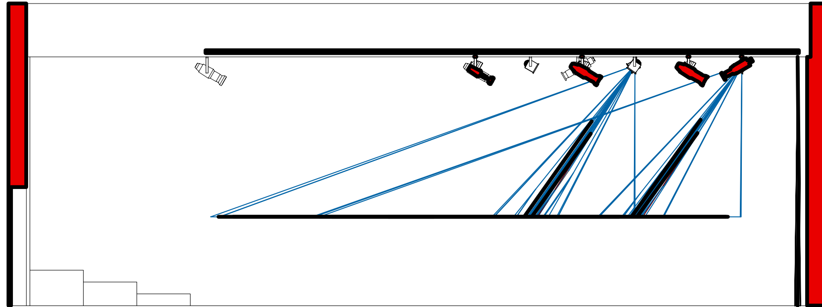
1 SR Section View Backlights Sht-6 Scale: 3/16" = 1'-0"
